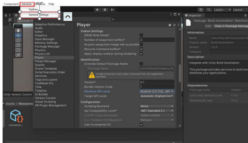
Figure 27. Android version settings.
