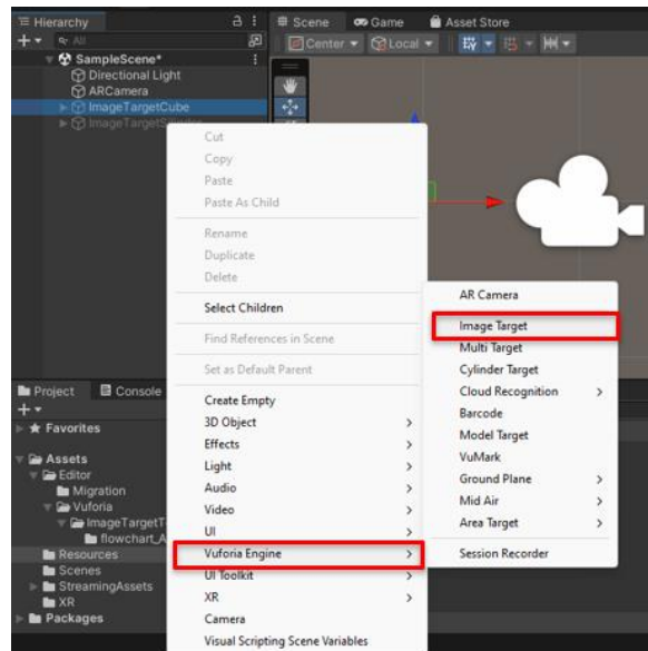
Figure 16. Create a game object.
