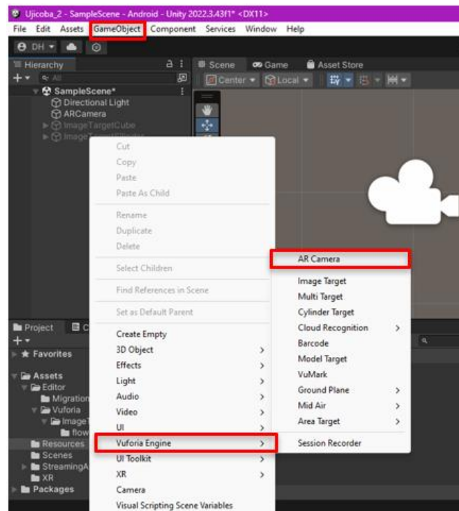
Figure 13. Using AR Camera and Delete Main Camera.
