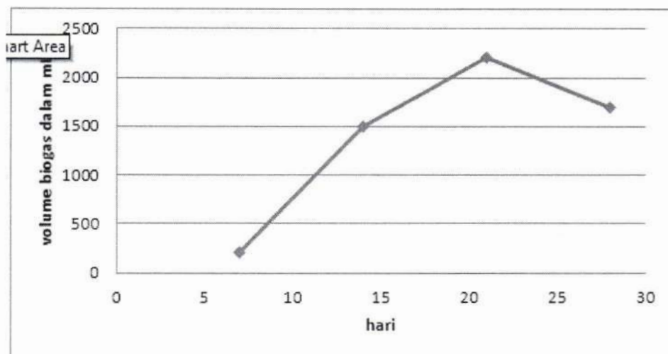
Gambar 5. Analisa volume biogas
